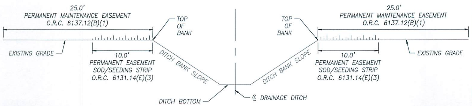
TYPICAL DRAINAGE IMPROVEMENT SECTION - OPEN DITCH
